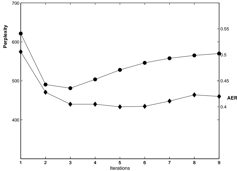
Figure 1: Training curve for ITG model, showing perplexity on cross-validation data, and alignment error rate on a separate hand-aligned dataset.
