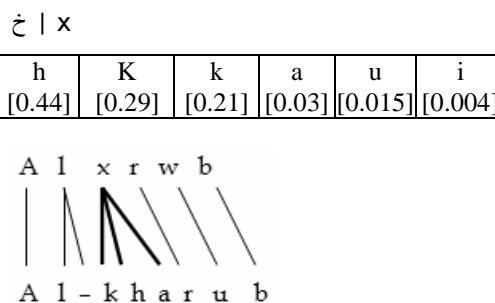
Figure 1. Example of the learned A-E character transliteration model with probabilities, and its application in the alignment between an Romanized Arabic name and an English translation.
