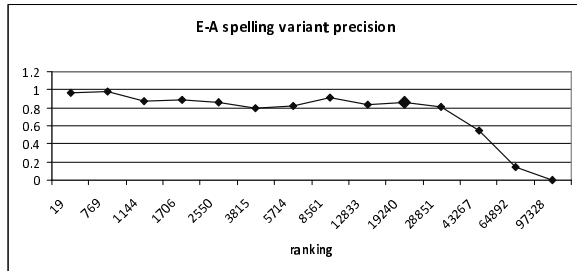
Figure 3. English-Arabic name spelling variants precision curve.
