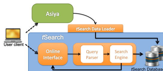
Figure 2: tSEARCH architecture
