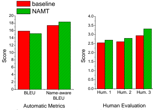
Figure 2: Scores based on Automatic Metrics and Human Evaluation.
