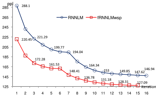
Figure 4: Convergence curve.
