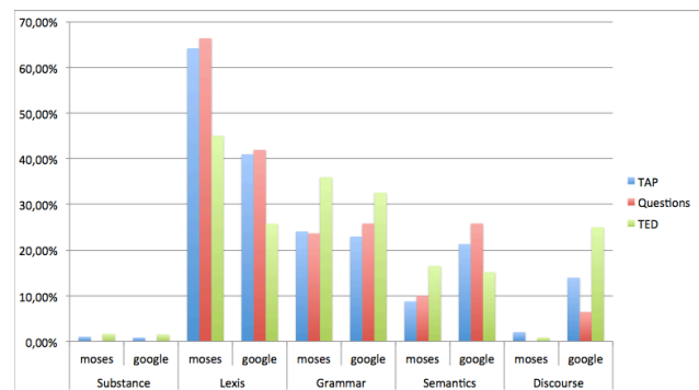
Figure 3: Errors in Moses and Google, by errors' type
