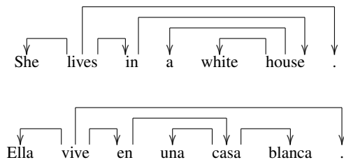
Figure 1: Projective Dependency Structures
