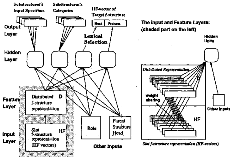
Fig. 2: Phrasal Network Structure: (a) the architecture of a phrasal network. (b) details of the lowest two layers. The unshaded slots represent the input f-structure. The shaded ones represent the context f-structure.
