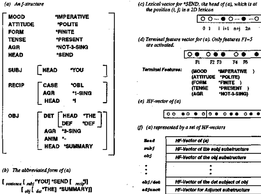
Fig. 1: F-structure representation: (a) an f-structure. (b) abbreviation. (c) lexical vector. (d) terminal feature vector. (e) HF-vector. (f) f-structure represented by HF-vectors.
