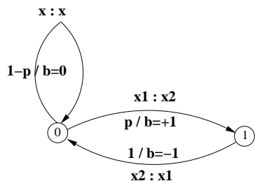
Figure 1: The uniform MJ1 reordering transducer.
