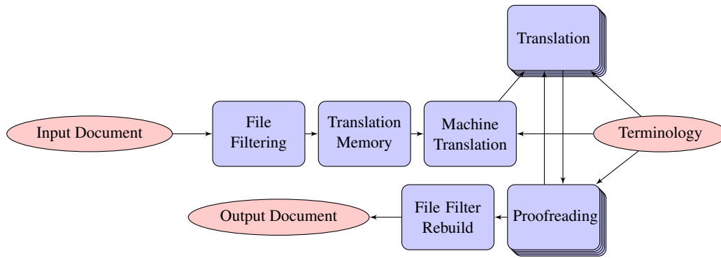
Figure 5: Possible translation workflow in SmartMATE
