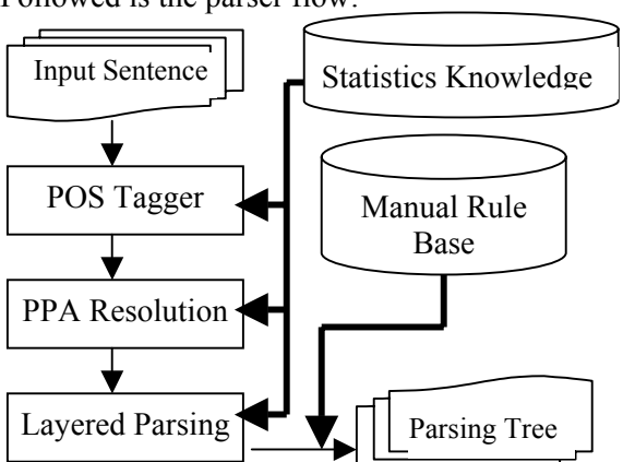
Figure 2. Parser based on Hybrid Methods
