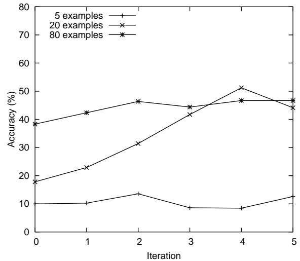
Figure 4: Proportion of correctly discovered NE pairs vs. the initial example set size. As long as the size is large enough, decreasing the number of examples does not have a significant impact on the performance of the later iterations.
