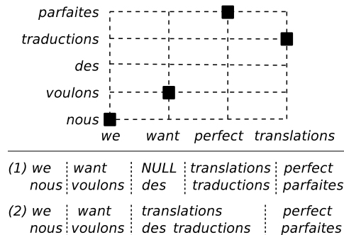
Figure 1: Tuple extraction from a sentence pair.
