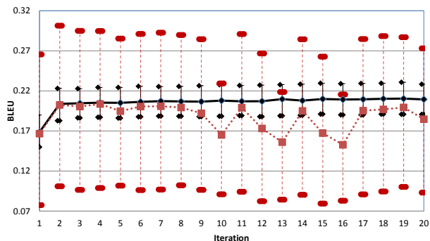
Figure 1: Comparison of performance on development set for cs-en when using LU/MC and M\pm C selection.
